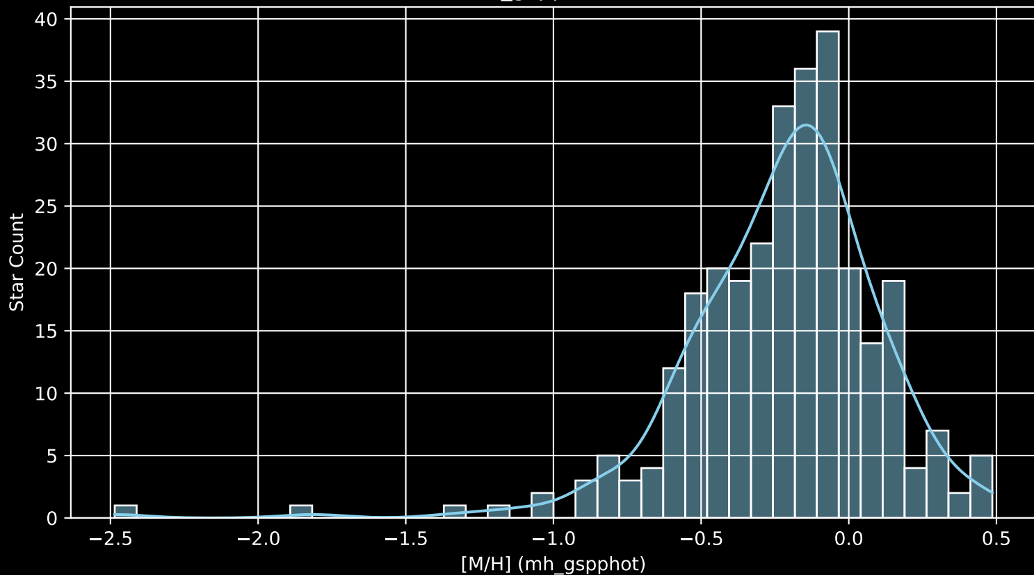
APOGEE DR17 Field: [063+44_MGA [M/H] (mh_gspphot) (n= 291)
