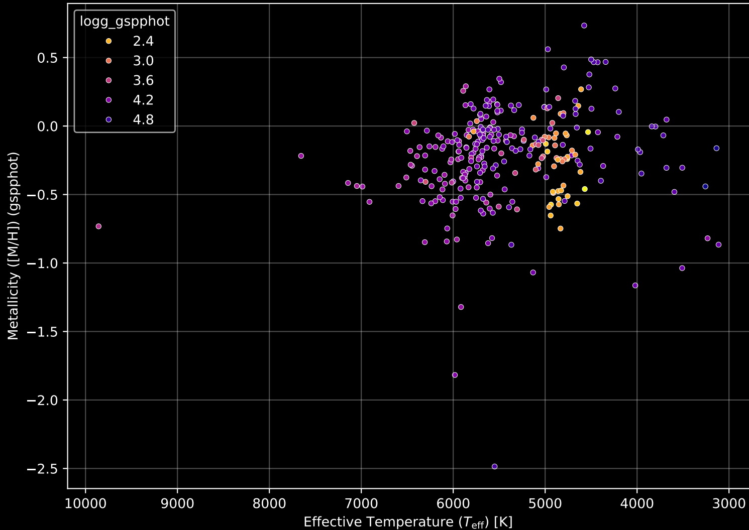
APOGEE DR17 Field: [063+44_MGA] Stellar Population Parameters (n= 293)
