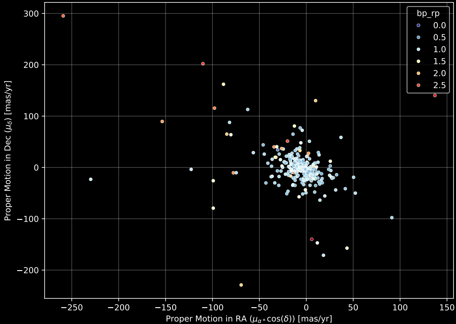
APOGEE DR17 Field: [063+44_MGA] Proper Motion Diagram (n= 293)
