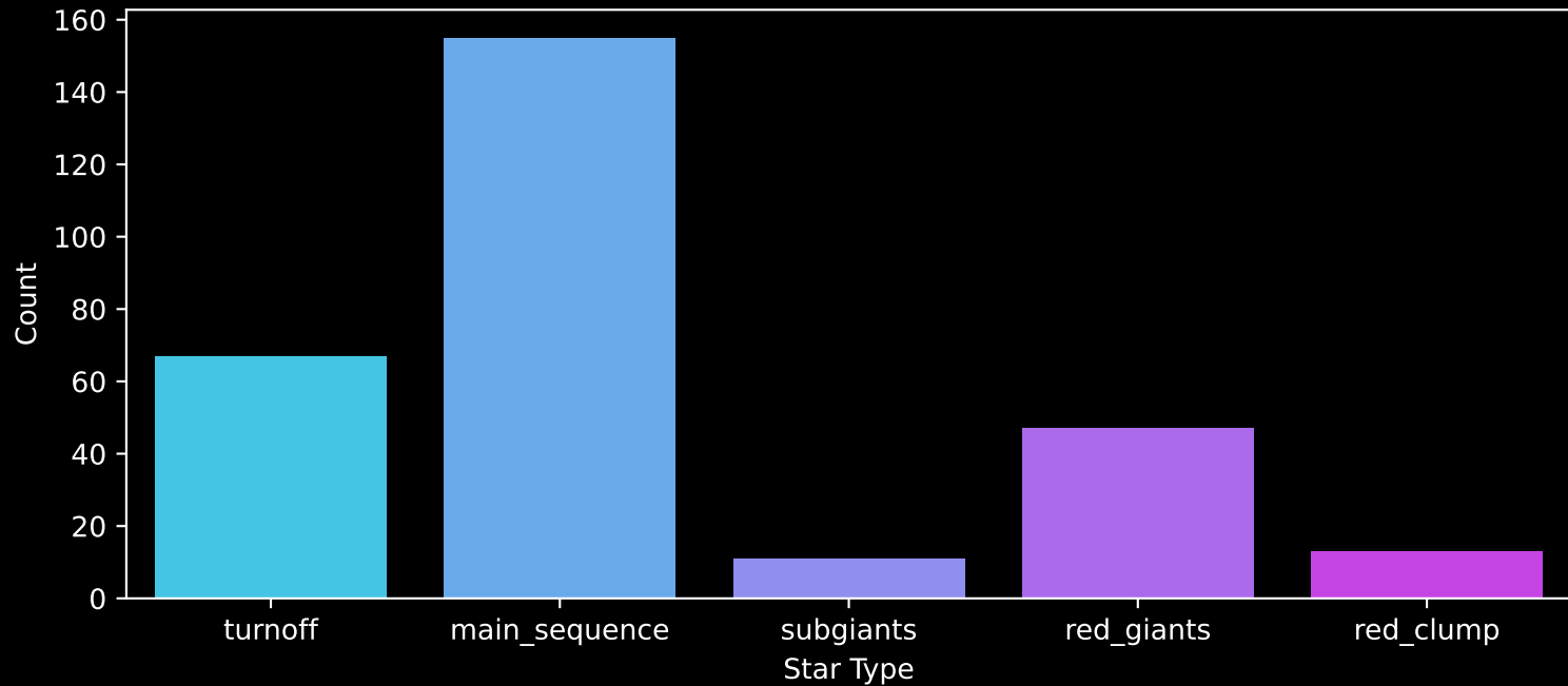
APOGEE DR17 Field: [063+44_MGA] Count plot of Star Type
