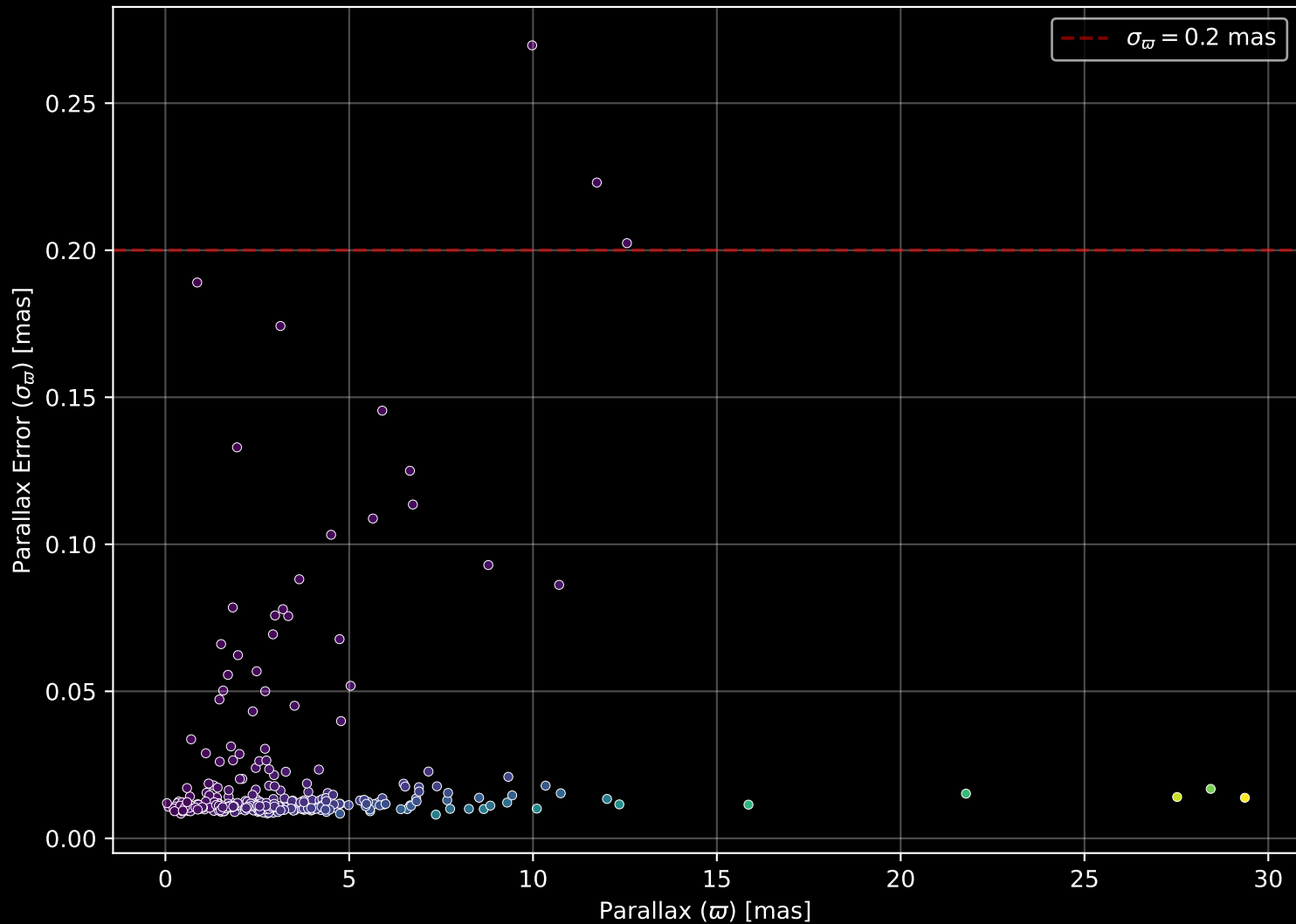
APOGEE DR17 Field: [063+44_MGA] Parallax Quality (n= 293)
