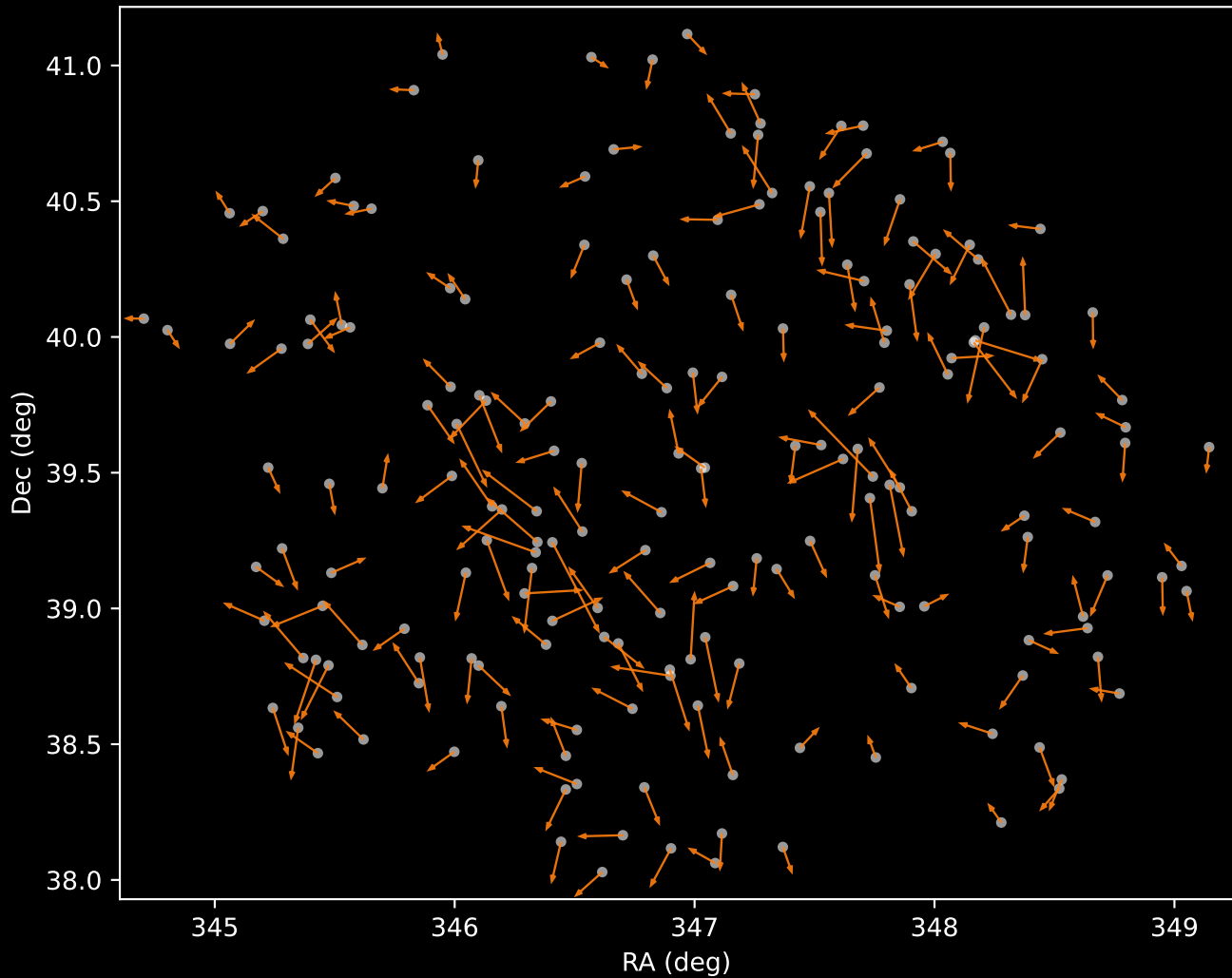
APOGEE DR17 Cluster 2 Proper Motion Vectors (n=189)
