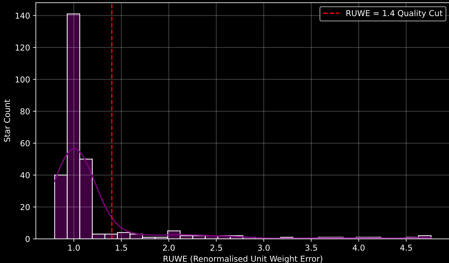
GAPOGEE DR17 Field [063+44_MGA] RUWE Distribution (n= 270)
